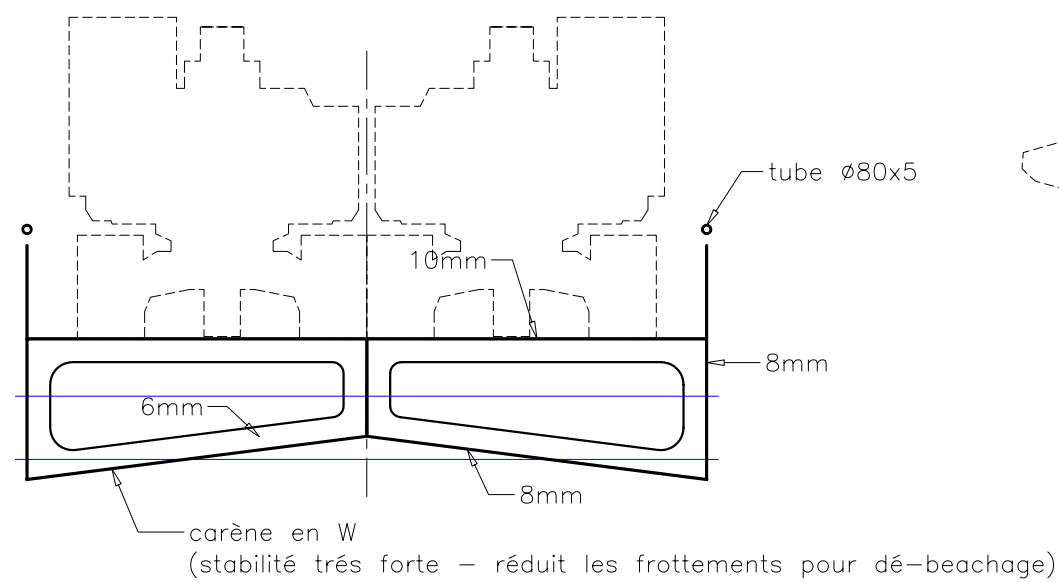
SECTION TYPE
